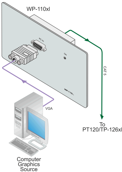
Figure 2: Connecting the WP-110xl UXGA/Data Line Transmitter
