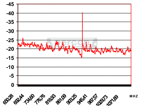
dB STRUCTURAL RETURN LOSS 650Mhz-1.1Ghz
