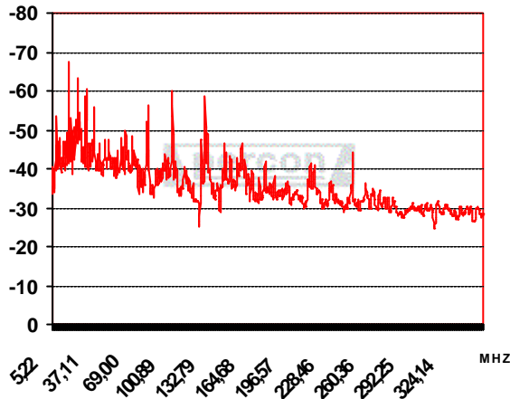
dB STRUCTURAL RETURN LOSS 5Mhz-300Mhz
