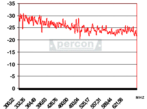
dB STRUCTURAL RETURN LOSS 300Mhz-650Mhz
