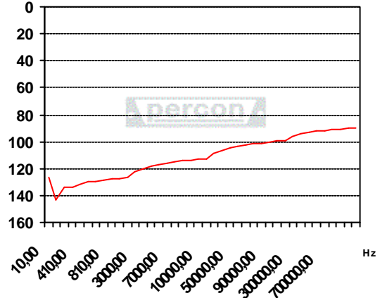
pF/m CAPACITANCE conductor to conductor
